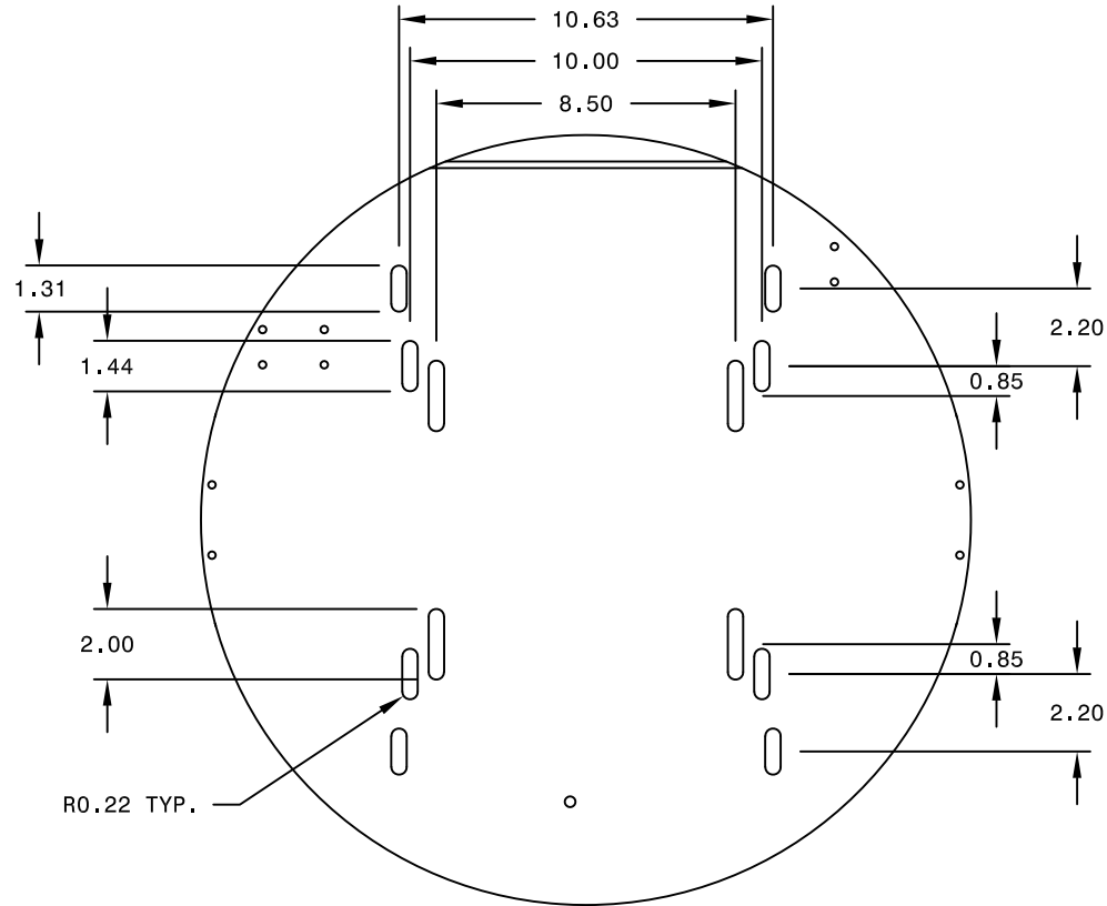
SECTION B C/T MOUNTING PROVISIONS
