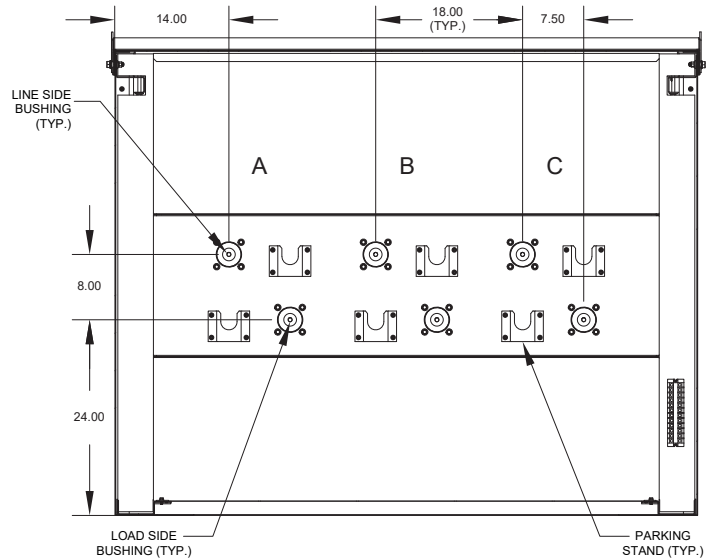
FRONT ELEVATION DOORS REMOVED (ONE IN / ONE OUT SHOWN)
