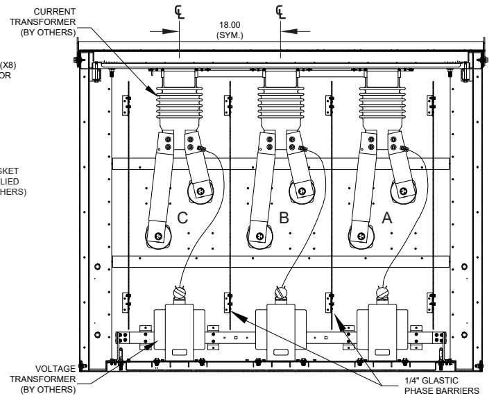
REAR ELEVATION DOORS & INCIDENTAL CONTACT BARRIERS REMOVED (ONE IN / ONE OUT SHOWN)
