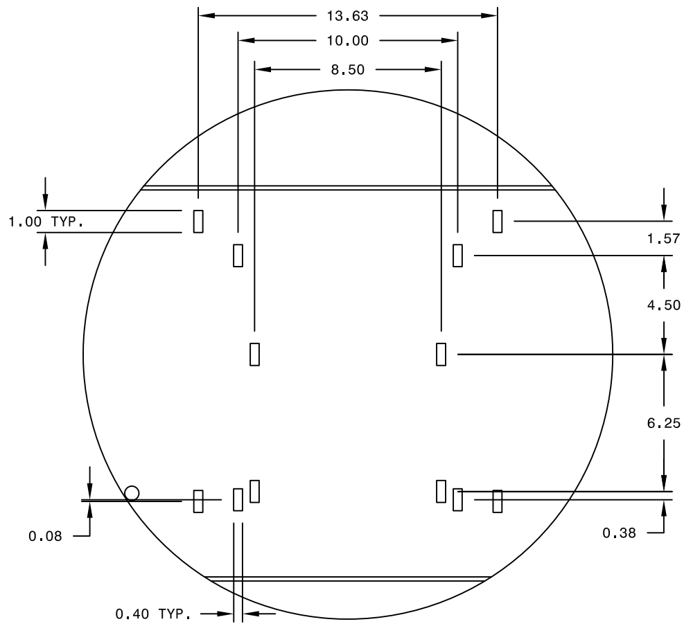
SECTION A V/T MOUNTING PROVISIONS
