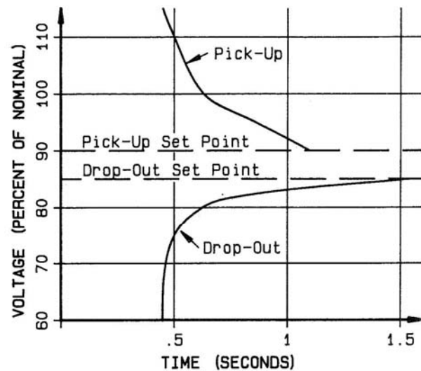
TIME DELAY CHARACTERISTICS OF A LAKE SHORE 3 PHASE VOLTAGE SENSING RELAY
