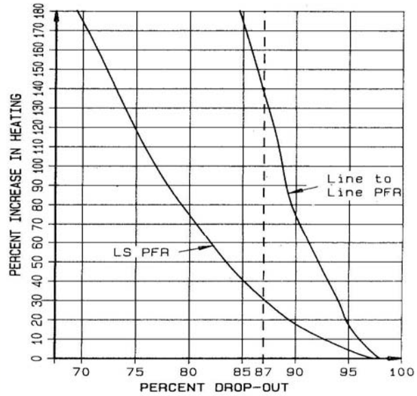
DROPOUT SETTING VERSUS PERCENT INCREASE IN MOTOR HEATING
