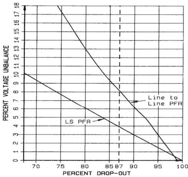
DROPOUT SETTING VERSUS PERCENT VOLTAGE UNBALANCE
